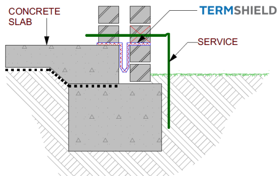
Details for the installation of TermShield stainless steel mesh at perimeter barrier to walls at Slab-on-ground.
