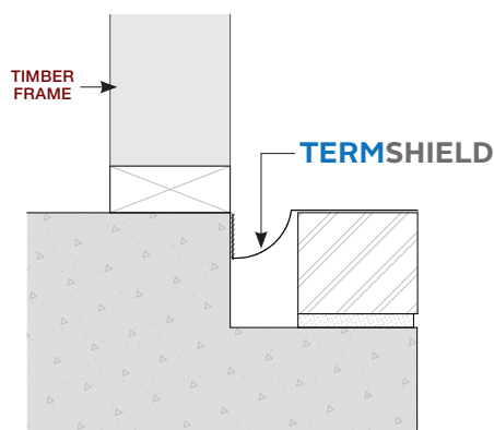
Details for the installation of TermShield brick veneer construction.
