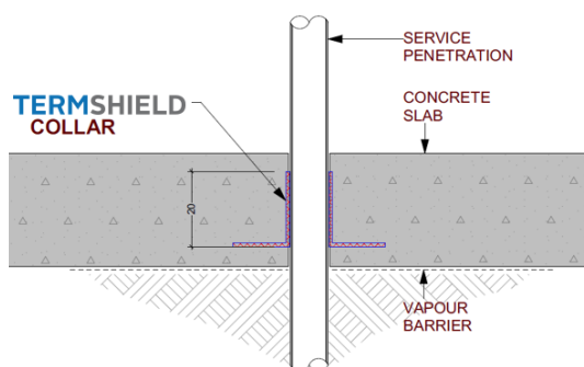
Details for the installation of TermShield at service penetration.
