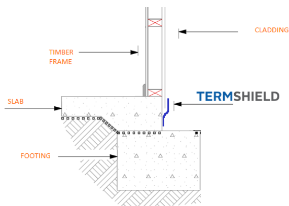
Details for the installation of TermShield at perimeter from slab to outer wall.
